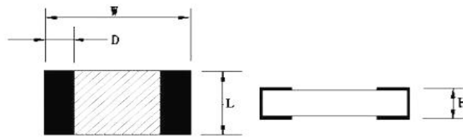
Chip Resistors Type B
