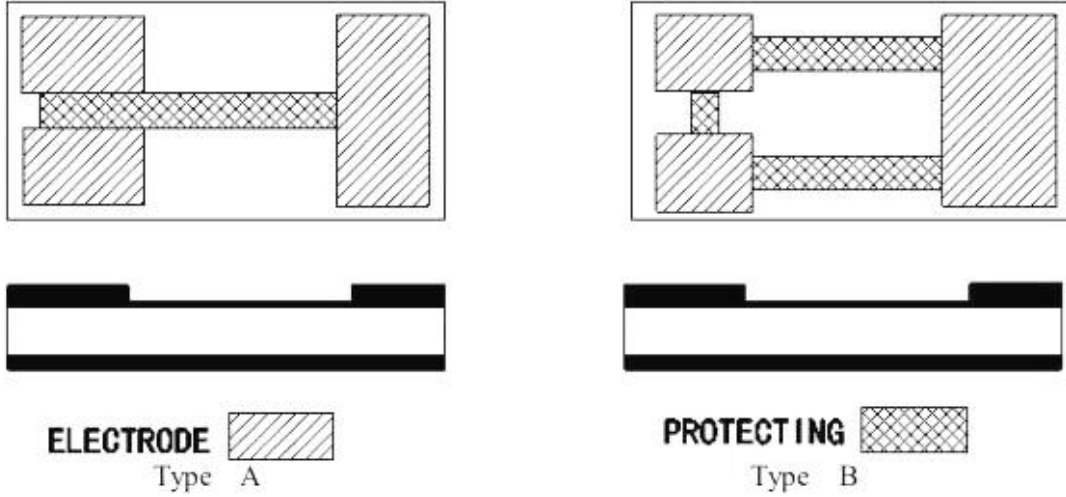
Outline Drawings
